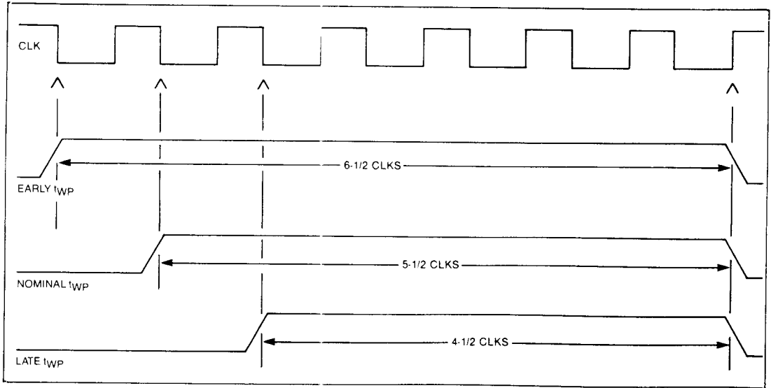
WRITE DATA TIMING
