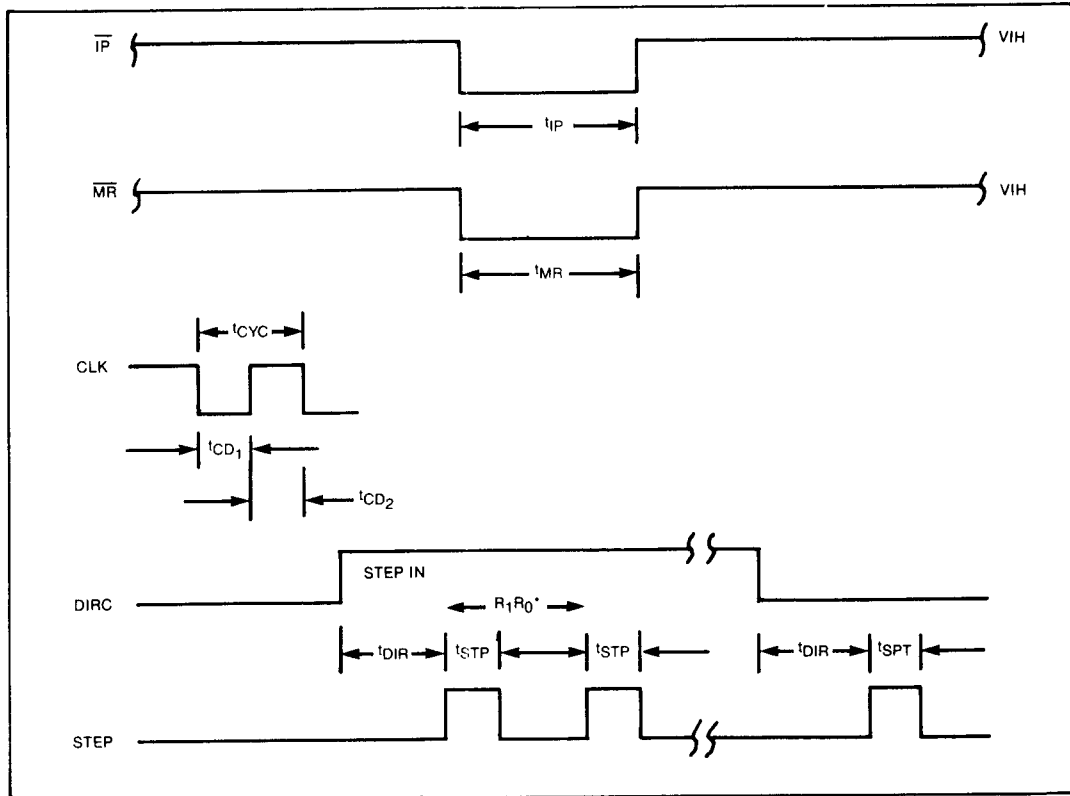
MISCELLANEOUS TIMING
