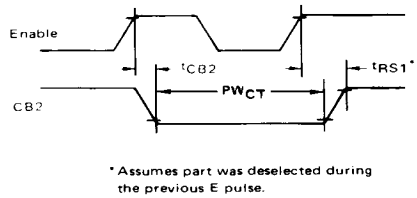
FIGURE 11 — CB2 DELAY TIME (Write Mode; CRB-5=CRB-3=1, CRB-4=0)
