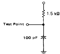
FIGURE 5 — NMOS EQUIVALENT TEST LOAD
