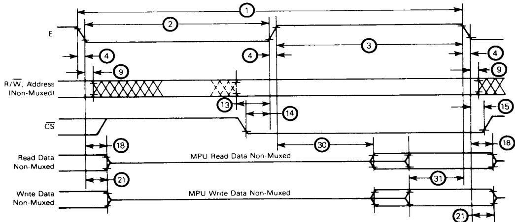
FIGURE 1 — BUS TIMING
