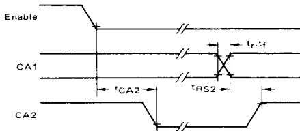
FIGURE 8 — CA2 DELAY TIME (Read Mode; CRA-5=1, CRA-3=CRA-4=0)
