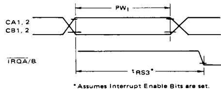
FIGURE 13 — INTERRUPT PULSE WIDTH AND \overline{IRQ} RESPONSE
