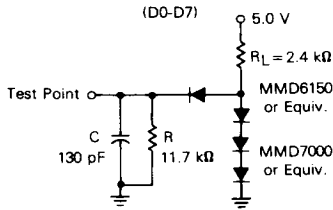
FIGURE 2 — BUS TIMING TEST LOADS
