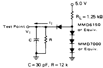
FIGURE 5 — NMOS EQUIVALENT TEST LOAD
