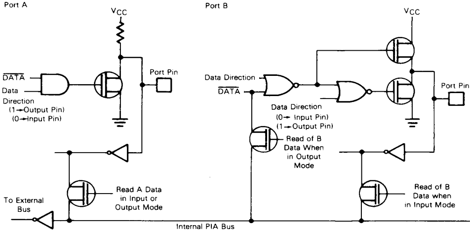
FIGURE 17 — PORT A AND PORT B EQUIVALENT CIRCUITS
