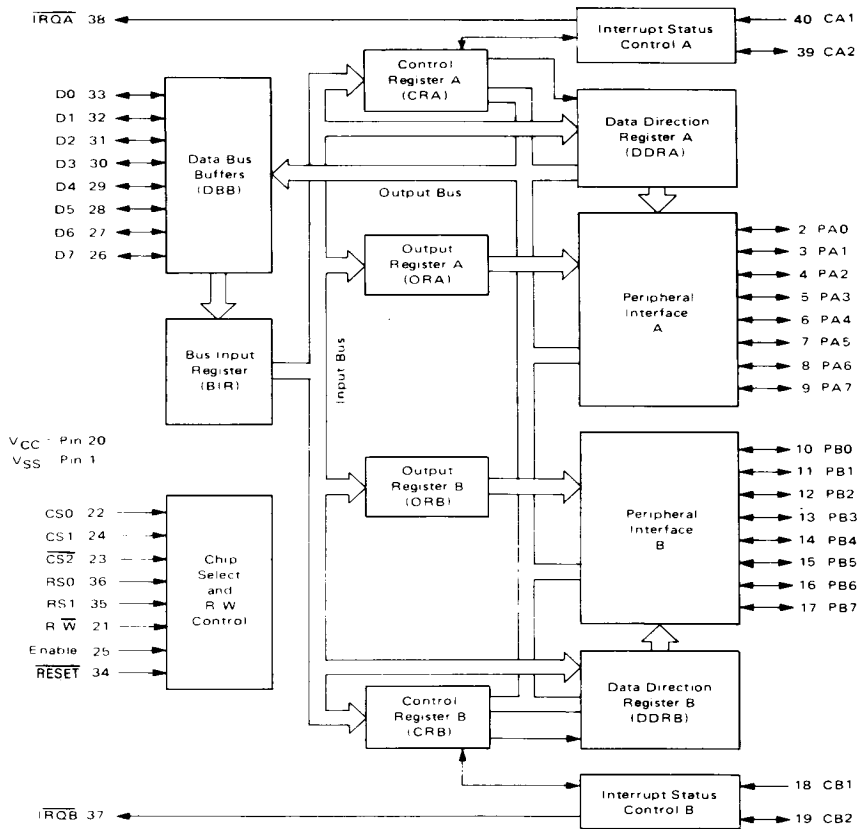
FIGURE 16 — EXPANDED BLOCK DIAGRAM
